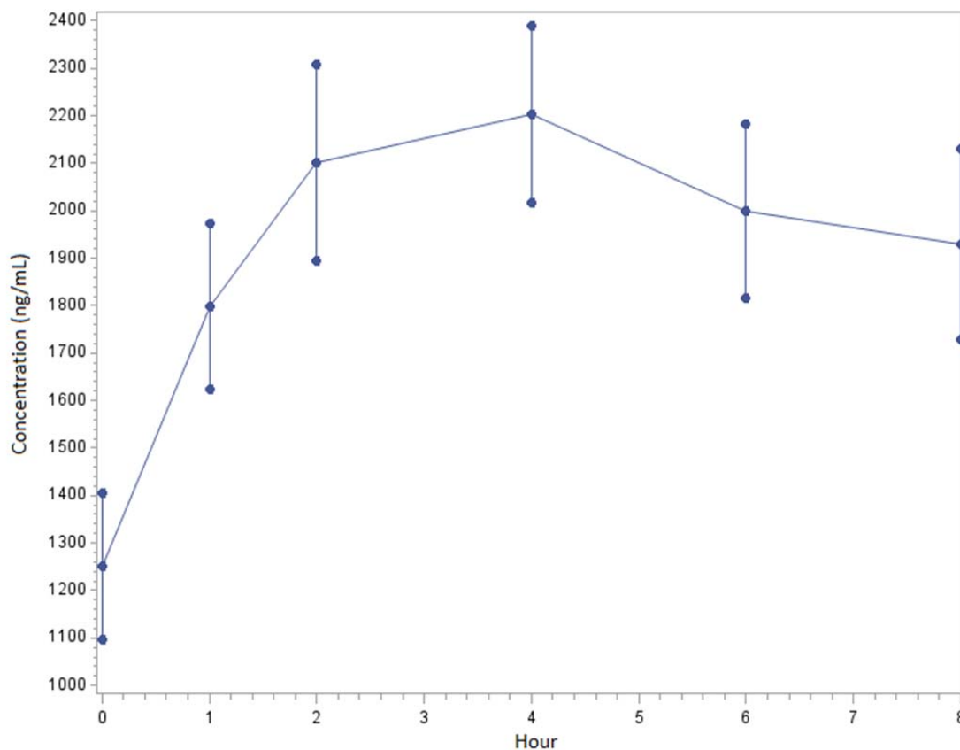
Figure S1 Lonafarnib pharmacokinetics. Mean plasma lonafarnib concentration (y axis) over an 8-h sampling period (x axis). Area under the curve 15.7 \pm 1.2 \mu\text{g} \cdot \text{h}^{-1} \cdot \text{mL}^{-1}
