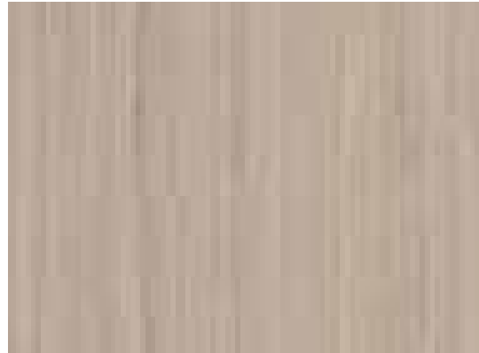
5232 | rocky ice
